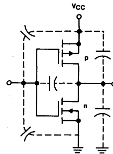
Fig. 2 - Parasitic capacitances in a CMOS inverter.
