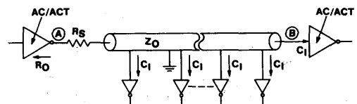
Fig. 44 - Transmission line feeding a number of AC/ACT inputs.
