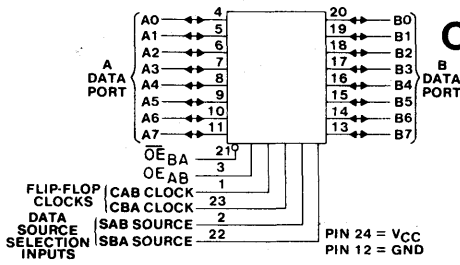
FUNCTIONAL DIAGRAM
