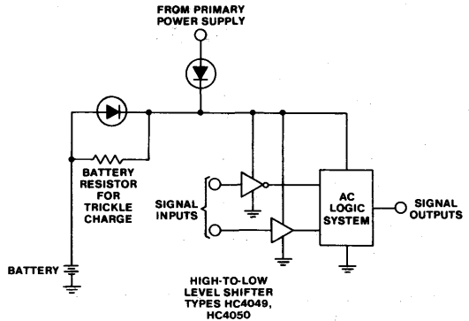
Fig. 61 - Example of AC/ACT system with battery back-up.
