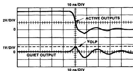
Fig. 26 - Simultaneous switching transient performance of an AC240 octal-type IC in a small-outline (SO) package. See Fig. 22 for test conditions.
