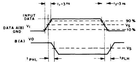
Fig. 3 - Propagation delay times.
