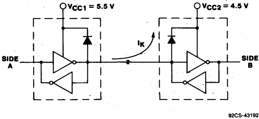
Fig. 59 - Dual power supply interface.
