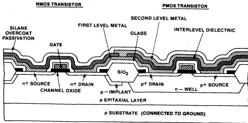
Fig. 1 - Cross section of AC/ACT two-level-metal CMOS process.
