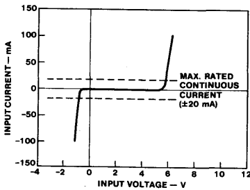
Fig. 6 - AC/ACT input characteristic.
