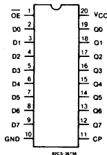
CD54/74AC/ACT574
