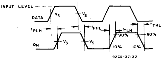
Fig. 3 - Data to Q_n output propagation delays.
