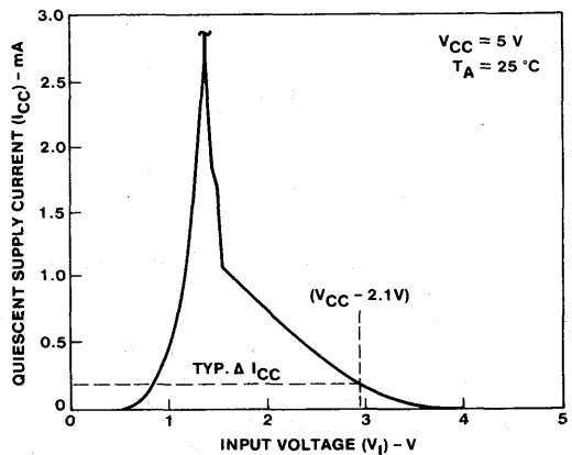
Fig. 36 - Quiescent supply current ( I_{CC} ) as a function of input voltage ( V_i ) for ACT types.
