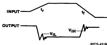
Fig. 38 - Results of typical input t_r , t_f tests on AC/ACT04/14 types. V_{cc} = 5 \text{ volts} . T_A = 25^\circ \text{C} . The maximum value of t_r , t_f is defined for condition that output ringing exceeds V_{IL} or goes below V_{IH} . Five of six outputs are switching simultaneously.
