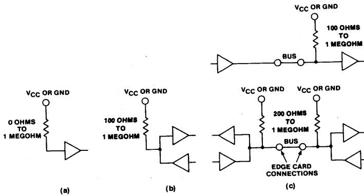
Fig. 53 - Input terminations for (a) unused logic inputs, (b) unused I/O ports inputs, and (c) used inputs coming off an edge card connector.
