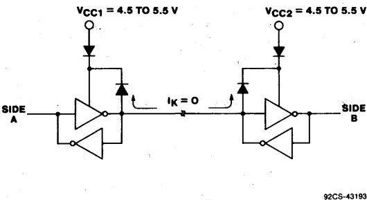
Fig. 60 - Blocking diodes in series with the V_{CC} supply pin of I/O buffers or transceivers ease multisupply interfacing.
