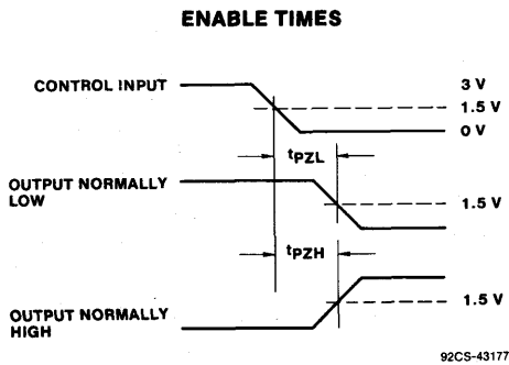
Fig. 84 - Output enable and disable times.
