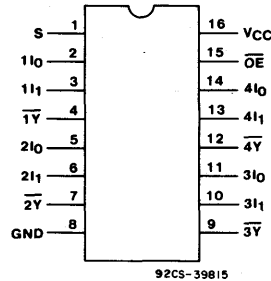
CD54/74AC/ACT258
