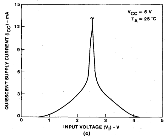
Fig. 35 - Quiescent supply current ( I_{CC} ) as a function of input voltage ( V_i ) for AC types.
