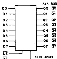
FUNCTIONAL DIAGRAM
