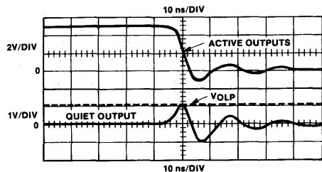
Fig. 25 - Simultaneous switching transient performance of an AC 240 octal-type IC in a dual-in-line package (DIP). See Fig. 22 for test conditions.
