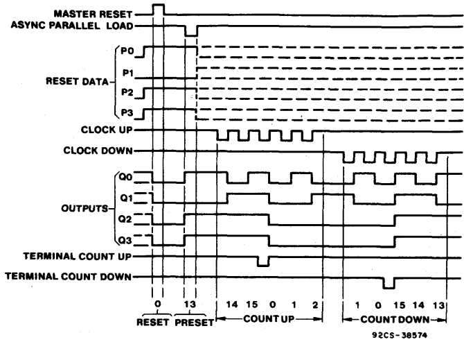
Fig. 2 - Timing diagram.
