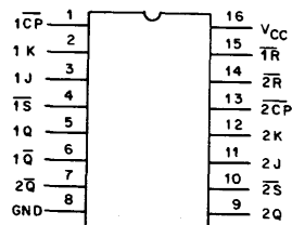
CD54/74AC/ACT112
