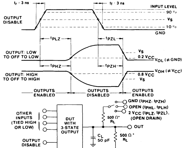
Fig. 2 - Three-state propagation delay waveforms and test circuit.
