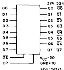
FUNCTIONAL DIAGRAM
