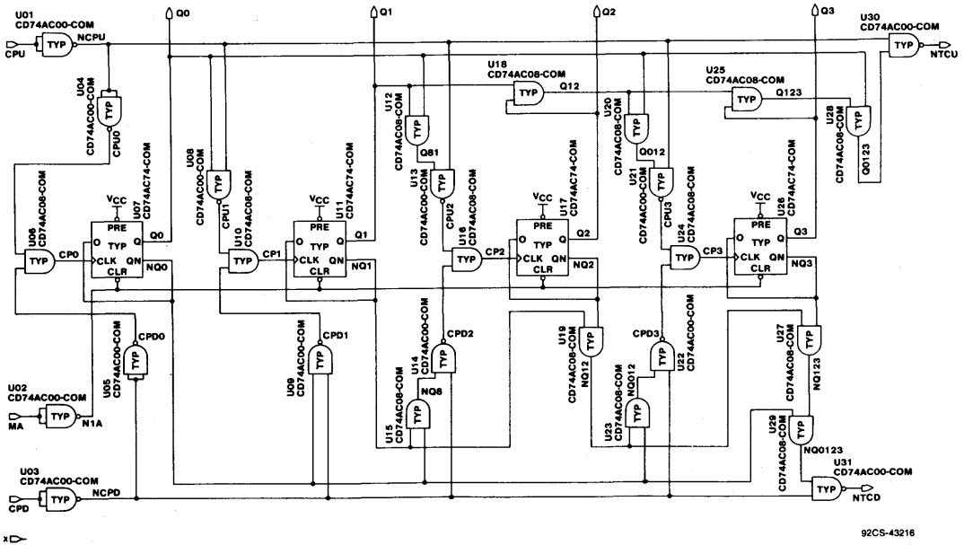
Fig. 65 - Schematic of AC193 4-bit up/down counter.
