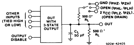
Fig. 2 - Three-state propagation delay waveforms and test circuit.
