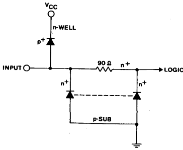
Fig. 5 - AC/ACT dual-diode input protection network.
