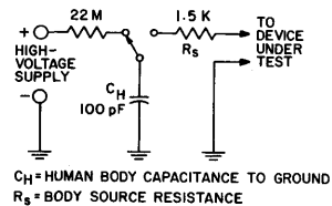
Fig. 8 - Test circuit for measuring electrostatic discharge (ESD) in AC/ACT circuits. The rise time at the output terminal should be 13 \pm 2 ns.
