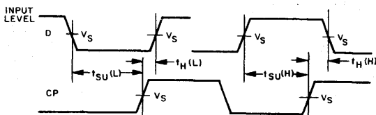
Fig. 3 - Prerequisite for clock.
