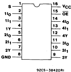
CD54/74AC/ACT257
