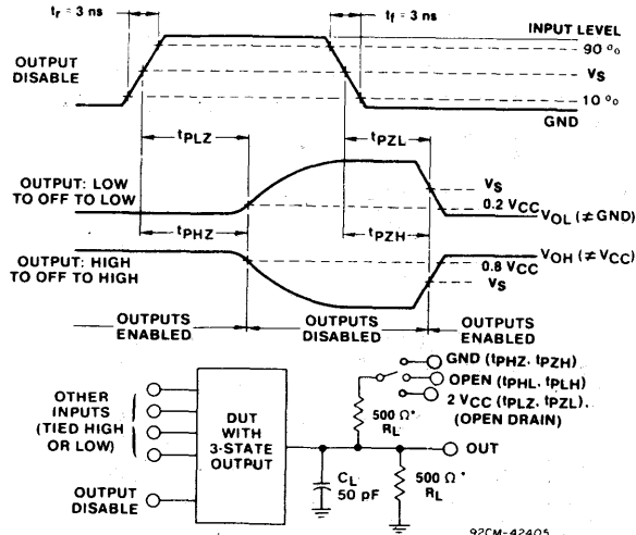
Fig. 1 - Three-state propagation delay waveforms and test circuit.
