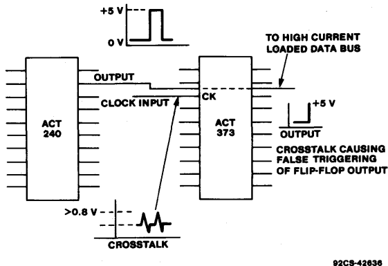
Fig. 76 - A poor layout showing a switching data bus driving a termination of 100 ohms or less. False triggering can be induced by crosstalk in this circuit. Avoid running high-current bus traces between any clock or strobe inputs.
