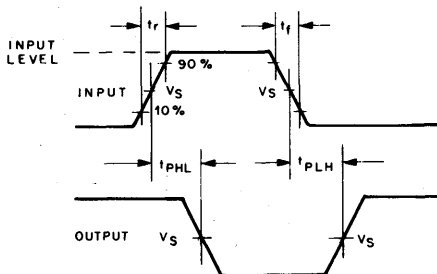
Fig. 1 - Propagation delay times and test circuit - AC/ACT04.
