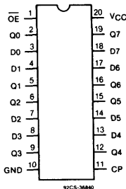
CD54/74AC/ACT374
