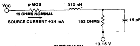
OUTPUT HIGH
