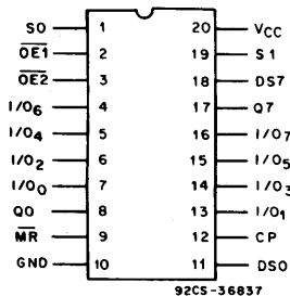
TERMINAL ASSIGNMENT
