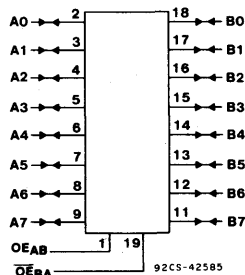
FUNCTIONAL DIAGRAM
