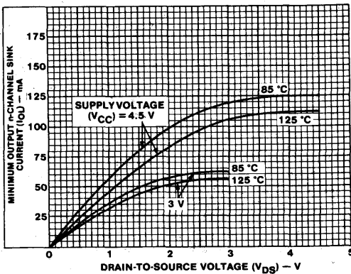
Fig. 18 - Minimum output characteristic curves at +85^\circ\text{C} and +125^\circ\text{C} for AC/ACT advanced high-speed CMOS types.
