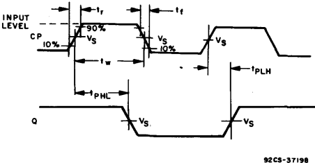
Fig. 1 - Propagation delay times and clock pulse width.
