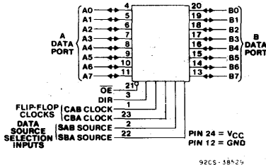
FUNCTIONAL DIAGRAM
