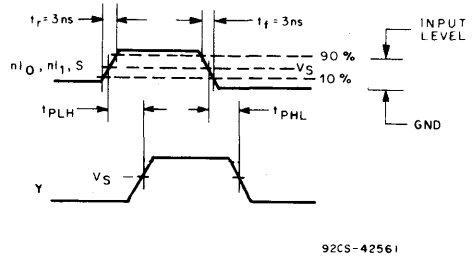
Fig. 3 - Inputs or select to output propagation delays (AC/ACT257).
