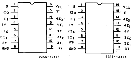
CD54/74AC/ACT157
