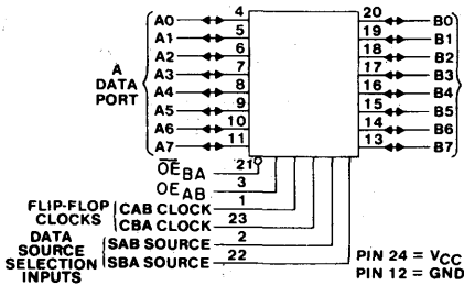
FUNCTIONAL DIAGRAM
