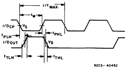
Fig. 7 - Waveforms showing the clock ( I/D_{CP} ) to output ( I/D_{OUT} ) propagation delays, clock pulse width, and maximum clock pulse frequency.
