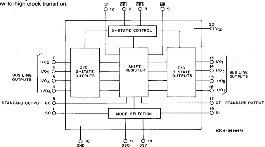
Fig. 1 - Functional diagram.
