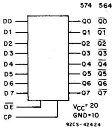
FUNCTIONAL DIAGRAM
