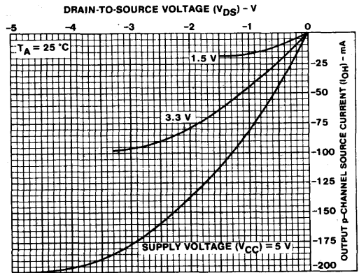
Fig. 17 - Minimum and typical output characteristics at +25^\circ\text{C} for AC/ACT advanced high-speed CMOS types.
