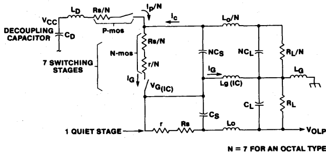
Fig. 23 - Equivalent circuit of ground-bounce configuration for an octal output stage. Dynamic value of R_S and transistor switch timing are key variables in minimizing ground bounce ( V_{OLP} ).
