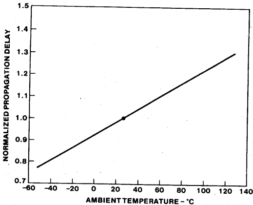
Fig. 30 - Normalized propagation delay as a function of ambient temperature for AC/ACT types.
