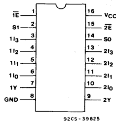
TERMINAL ASSIGNMENT
