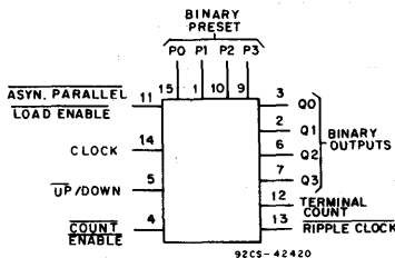
FUNCTIONAL DIAGRAM
