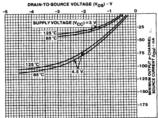
Fig. 18 - Minimum output characteristic curves at +85^\circ\text{C} and +125^\circ\text{C} for AC/ACT advanced high-speed CMOS types.
