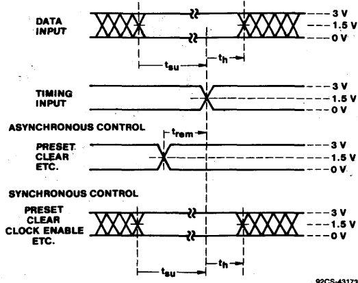
Fig. 83 - Setup, hold, and removal times.
