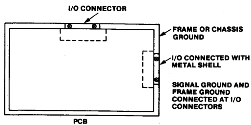
Fig. 77 - Preferred cable grounding.
