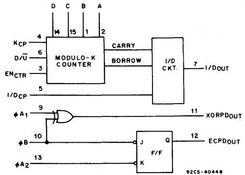
FUNCTIONAL DIAGRAM
