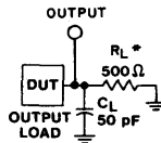
Fig. 3 - Propagation delay times and test circuit.
