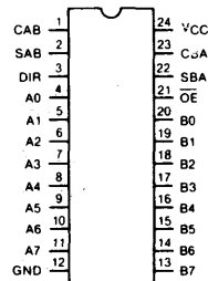
TERMINAL ASSIGNMENT
