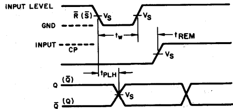
Fig. 2 - Reset or Set prerequisite and propagation delays.
