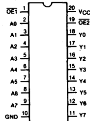
CD54/74AC/ACT541
