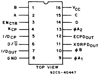
TERMINAL ASSIGNMENT
