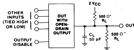
Fig. 3 - Open-drain propagation delay times and test circuit (A outputs).
