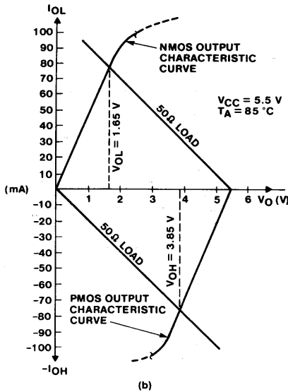
Fig. 48 - (a) Unterminated interconnection using AC types at line receive end. No shunt termination is required. (b) Plot of AC/ACT output driving 50-ohm line. (c) Waveforms for 8-inch board stripline. (d) Waveforms for 8-inch board stripline with added 470-ohm shunt termination resistance to dampen ringing.
