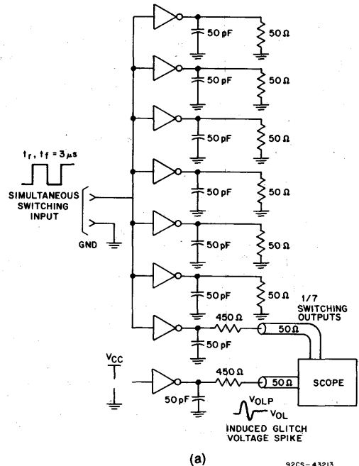
Fig. 21 - Ground lift caused by switching current transients through inductances described in Fig. 20.
