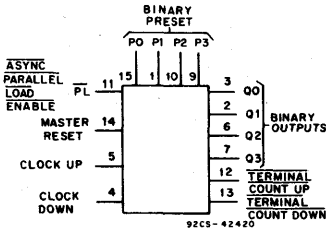
FUNCTIONAL DIAGRAM
