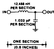
Fig. 2(a) - Cascade of 0.1-inch microstrip-line elements used to simulate each 0.8-inch of a slot-to-slot line segment.
