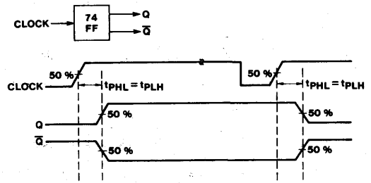
Fig. 33 - Delay balance of dual D-type flip-flop (74AC/ACT74).
