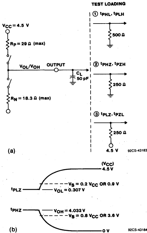
Fig. 32 - AC/ACT three-state test circuit and associated waveforms. (a) Output stage and the three JEDEC and RCA test load circuits, T_A = 85^\circ C . (b) Three-state output waveforms and test points. The RC time constant is a balanced 250 ohms and 50 picofarads.
