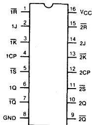
CD54/74AC/ACT109
