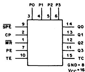
FUNCTIONAL DIAGRAM
