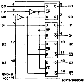
FUNCTIONAL DIAGRAM
