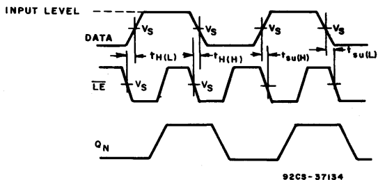
Fig. 5 - Latch enable prerequisite times.
