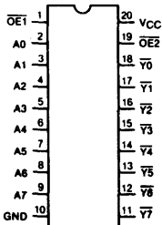
CD54/74AC/ACT540
