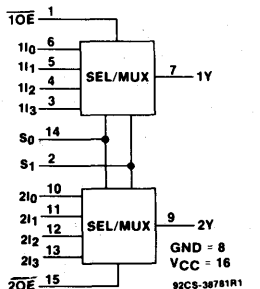
FUNCTIONAL DIAGRAM
