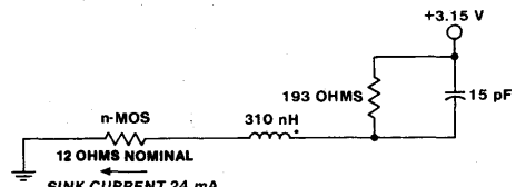
OUTPUT LOW
