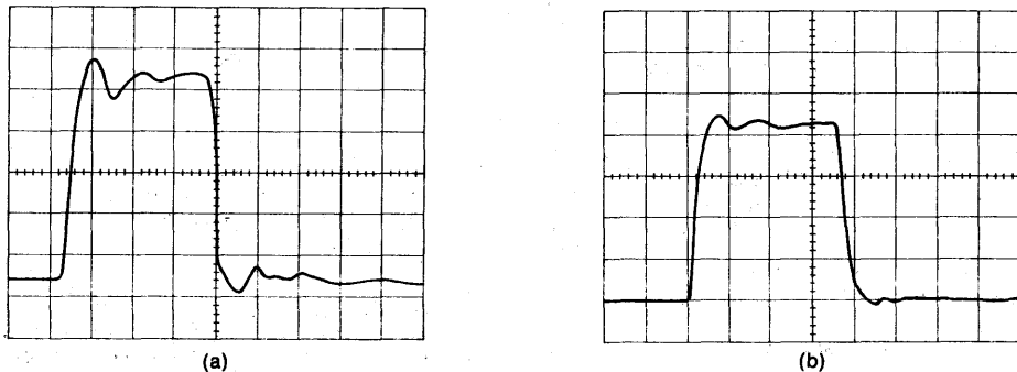
Fig. 42 - Buffer output with pure capacitive and pure resistive load makes a difference in ringing amplitude. One output switching. (a) R_L = 500 \text{ ohms} ; C_L = 15 \text{ picofarads} ( F.0 = 2 - 3 ) worst case. Overshoot = 0.6 volt; Undershoot = -0.4 volt (diodes help). (b) R_L = 100 \text{ ohms} (driving a resistive line); good case and very often applicable.
